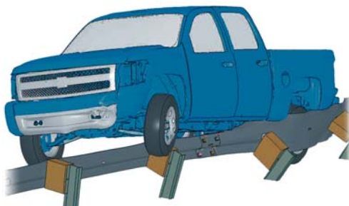
Road Side Model By courtesy of University of Nebraska
