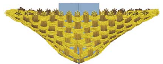
Detailed Model of Fabric By courtesy of ITV Denknendorf
