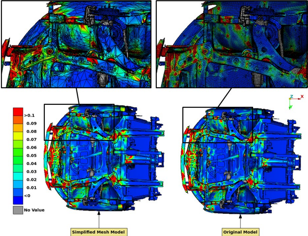
Fig.5 : Mesh simplification for shell surfaces
