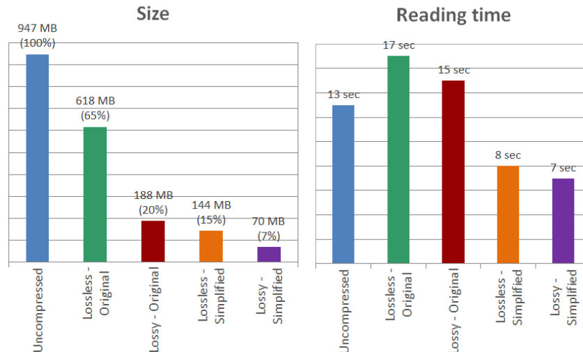
Fig.6 : Comparison of original / mesh simplified META databases
