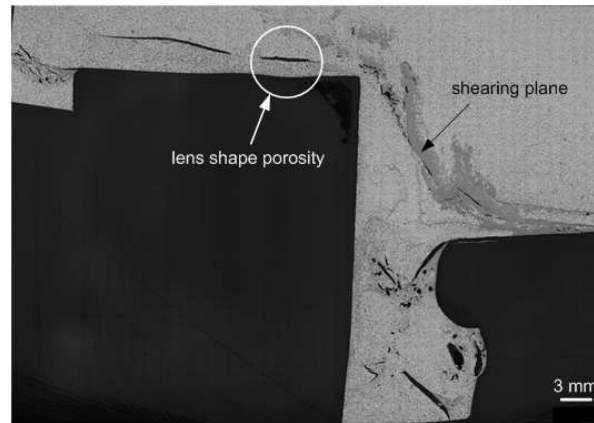
Figure 1: Porosity lens defects along a shearing plane
