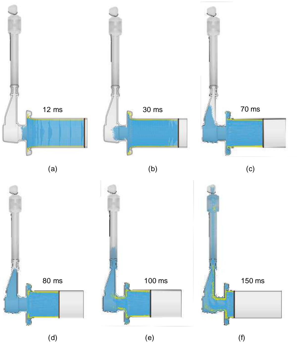
Figure 3: filling sequence, case 1
