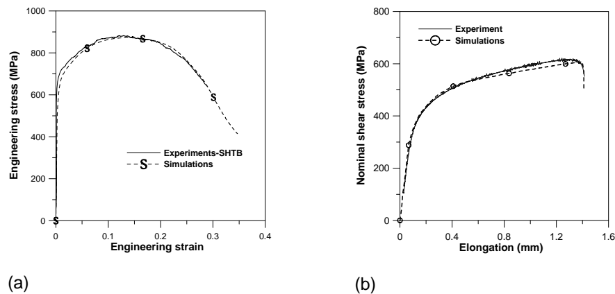
Figure 8. Comparison of experimental and numerical responses of (a) dynamic tensile test at 445 \text{ s}^{-1} , and (b) Shear test.
