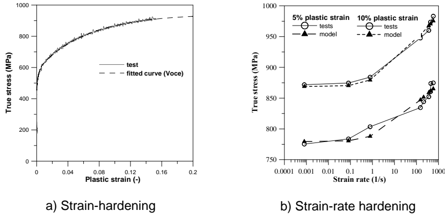
Figure 7. Comparison of test curves and fitted curve by Eq. (1).
